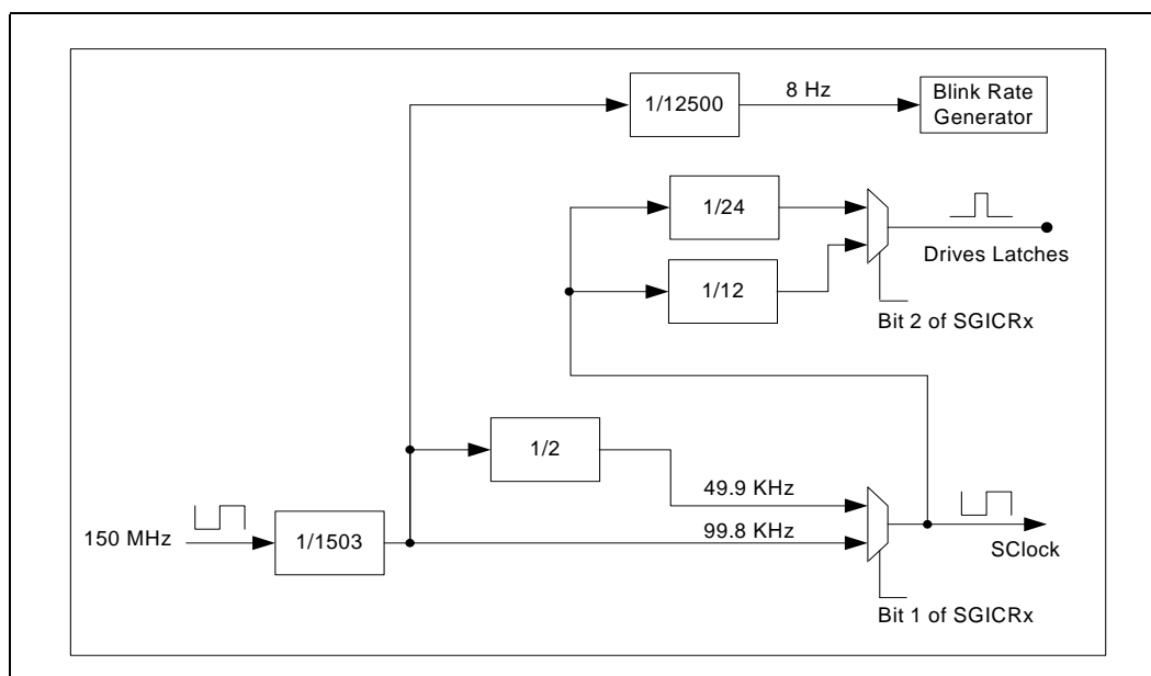
Figure 5-23. Clock Structure
