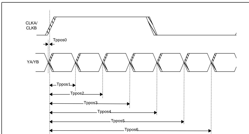
Figure 8-11. Clock Timing
