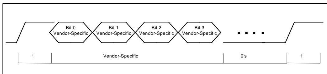
Figure 5-20. SLoad Signal
